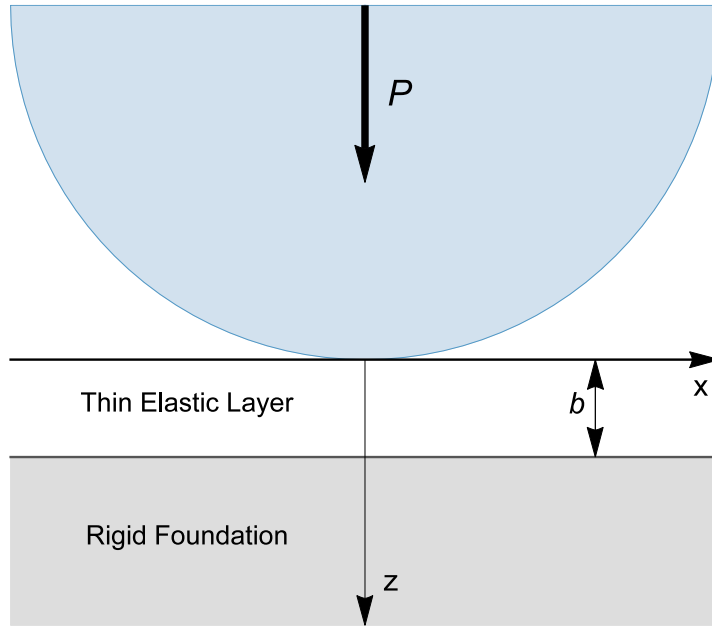
Fig. 1. The geometry for a rigid cylinder indenting a layer supported by a rigid foundation
