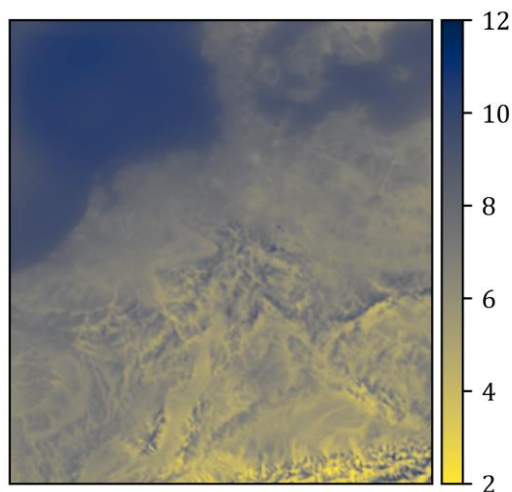
Figure 14: Mean wind speed at 122.32 m distribution 2008 in the data set in m/s. Every pixel represents a \sim 2.8 \times 2.8 km grid cell.
