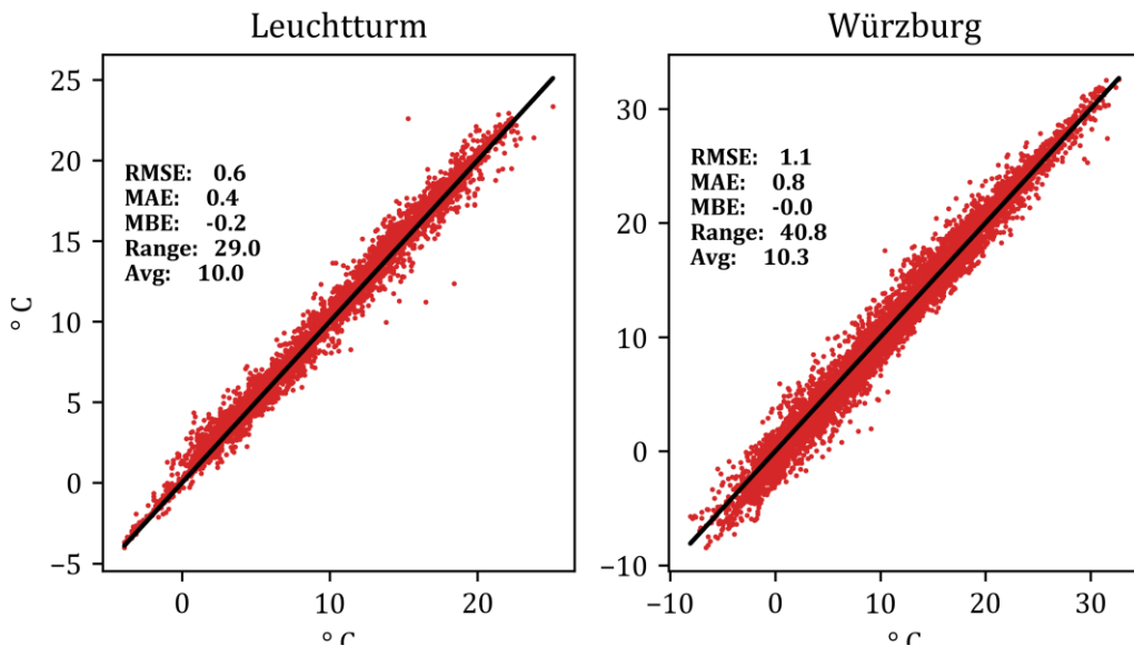
Figure 6: Best fits of COSMO data and observation data. The best in RMSE and MAE is Leuchtturm and in |MBE| Würzburg.
