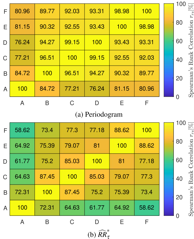
Figure 5. Similarity of PSD estimation for all pairs of system configurations as Spearman's rank correlation r_{rs} .
