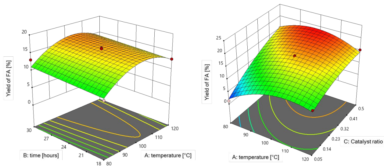
Figure 11: The 3D response surfaces for FA-yield as result of the Box-Behnken DoE. The red dots depict the run points above the surface and the pink dots depict the run points below the surface.
