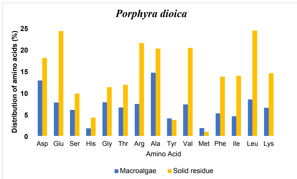
Figure 6: Amino acid profile for the macroalgae Porphyra dioica and its solid residue after the OxFA process. Reaction conditions: initial temperature 90 °C, non-isothermal reaction, 30 bar oxygen pressure, 1000 rpm stirrer speed, 24 h reaction time. The liquid phase consisted of 200 g of water with 10 g suspended macroalgae and 1.95 g of dissolved catalyst (1 mmol, HPA-2).
