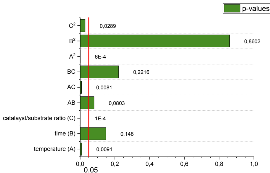
Figure 10: Pareto chart resulting of the Box-Behnken DoE for the quadratic model for the FA-yield. Red line indicates the significance level of p = 0.05 which shows if the value is significant or not. A value below the significance level is significant.
