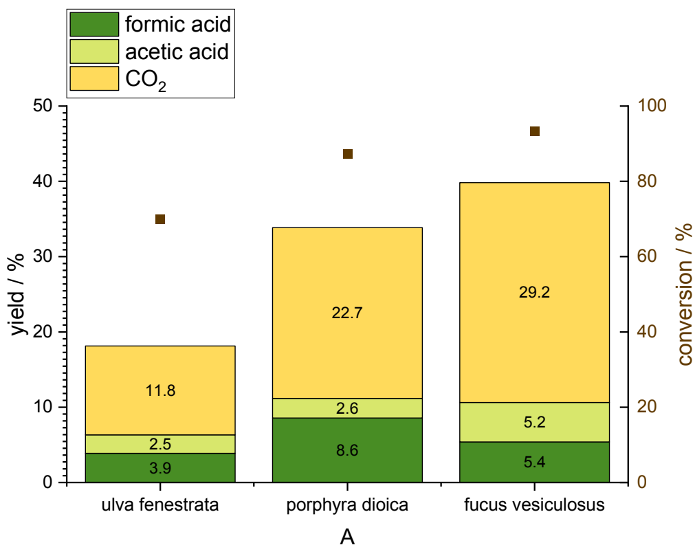
Figure 5: Screening of different macroalgae in the OxFA process for their product yield (left y-axis) and algae conversion (right y-axis) using the HPA-2 catalyst. Reaction conditions: HPA-2 at initial temperature 90 °C, non-isothermal reaction, 30 bar oxygen pressure, 1000 rpm stirrer speed, 24 h reaction time. The liquid phase consisted of 200 g of water with 10 g suspended macroalgae and 1.95 g of dissolved catalyst (1 mmol, HPA-2).
