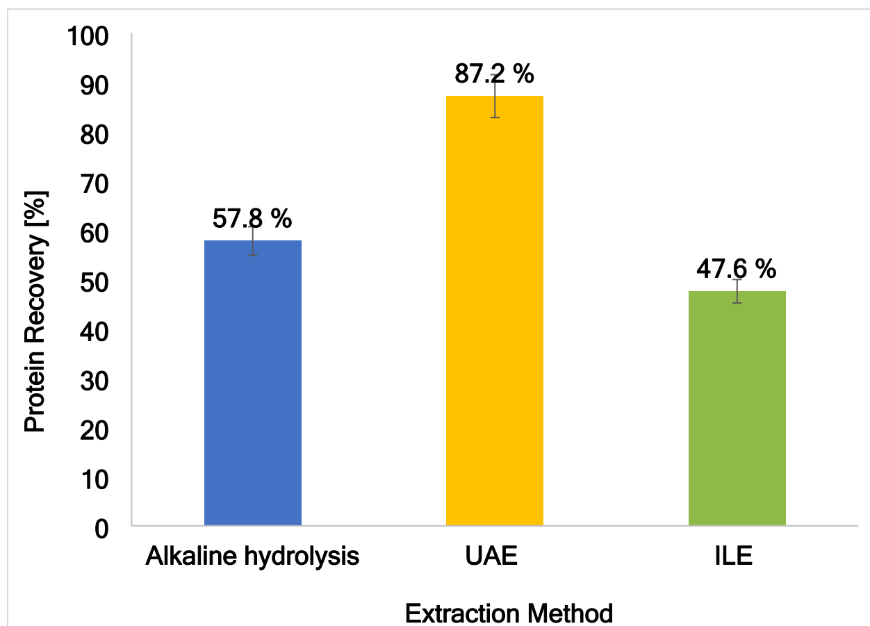
Figure 17: The mean protein recovery from the solid residue after the OxFA process is presented. Comparison of the three methods alkaline hydrolysis (at 0.1 M NaOH), UAE (at 100 % power input), and ILE (at 50 wt. % CCl 4 ) is shown. The highest protein recovery was compared in each case.
