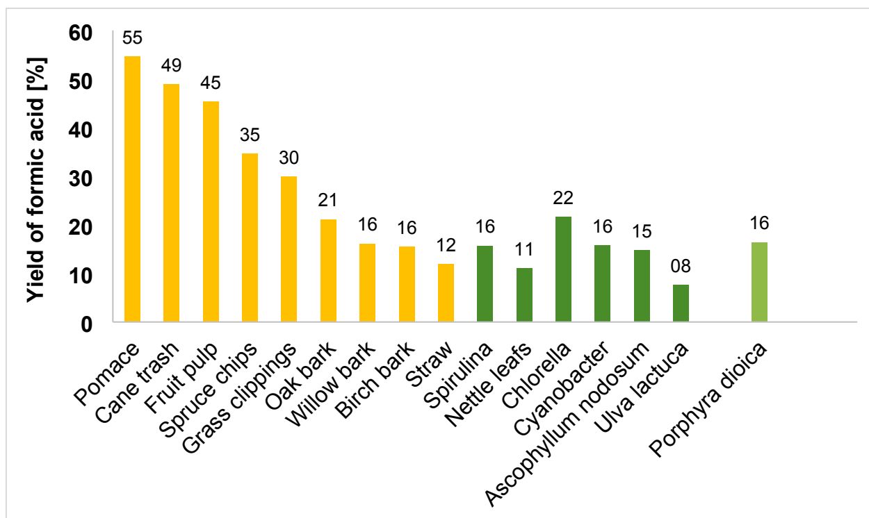
Figure 13: Graph for comparing the FA-yield for different biomass substrates for the OxFA process. (yellow and dark green: Reaction conditions: 3.3 g substrate, 1.9 g (11 mmol) additive para- toluene sulfonic acid and 1.74 g (0.9 mmol) HPA-2 catalyst dissolved in 100.0 mL H 2 O, 30 bar O 2 , 90 °C, 24 h, 1000 rpm; 27 light green: optimized reaction conditions for protein and FA production from Porphyra dioica : 80 °C, 30 h, 0.5 g catalyst /g substrate , 30 bar oxygen pressure, 1000 rpm stirrer speed, 10 g of Porphyra dioica as substrate, 200 mL of water as solvent.
