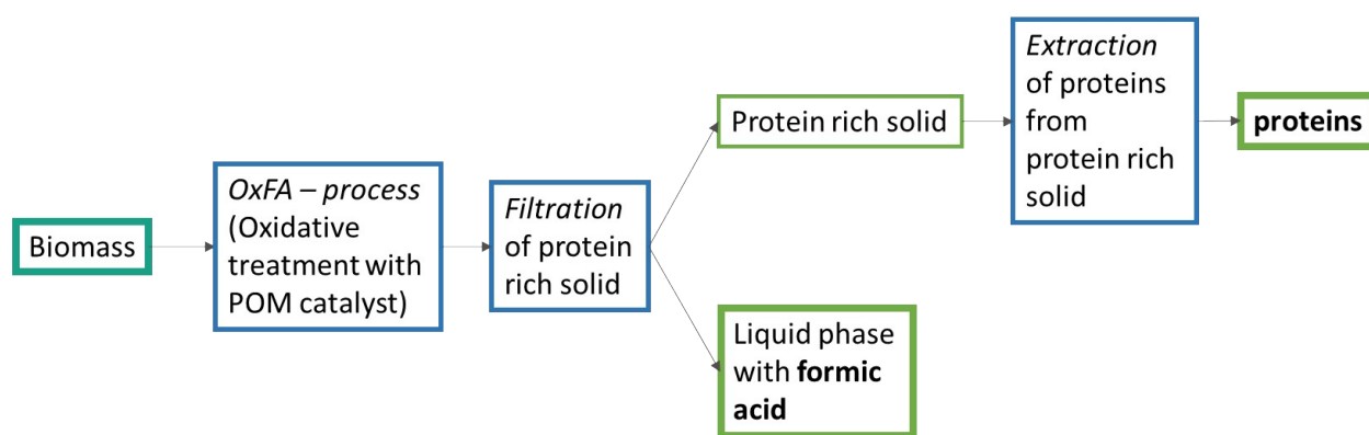
Figure 1: Schematic flow-chart of the ProFA process. The unit operations are marked in blue and the reactants and products are colored greenish.
