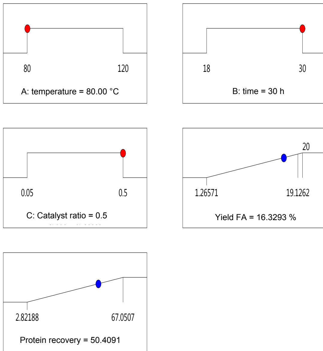
Figure 12: The optimized conditions resulting from the Box-Behnken DoE maximizing FA-yield as well as protein recovery.
