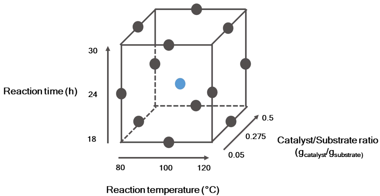
Figure 2: Parameter room for the designed Box-Behnken-DoE. The ranges of variables used are found at the edges.
