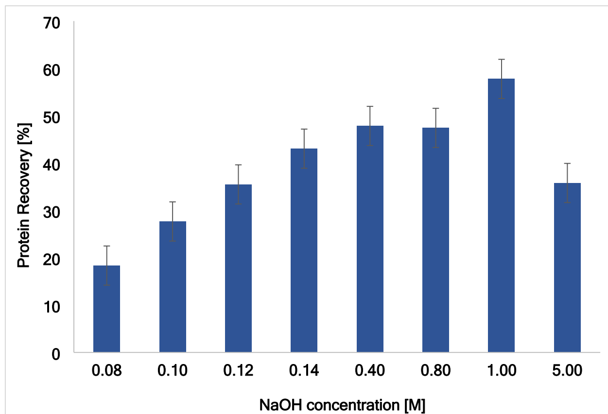
Figure 14: The mean protein recovery of alkaline hydrolysis from the solid residue after the OxFA process for the concentration of NaOH from 0.08 M to 5 M. Reaction conditions OxFA process: 30 bar oxygen pressure, 1000 rpm stirrer speed, 30 h reaction time, 80 °C, 200 g of water with 10 g suspended macroalgae and a catalyst/substrate ratio of 0.5, catalyst: HPA-2.
