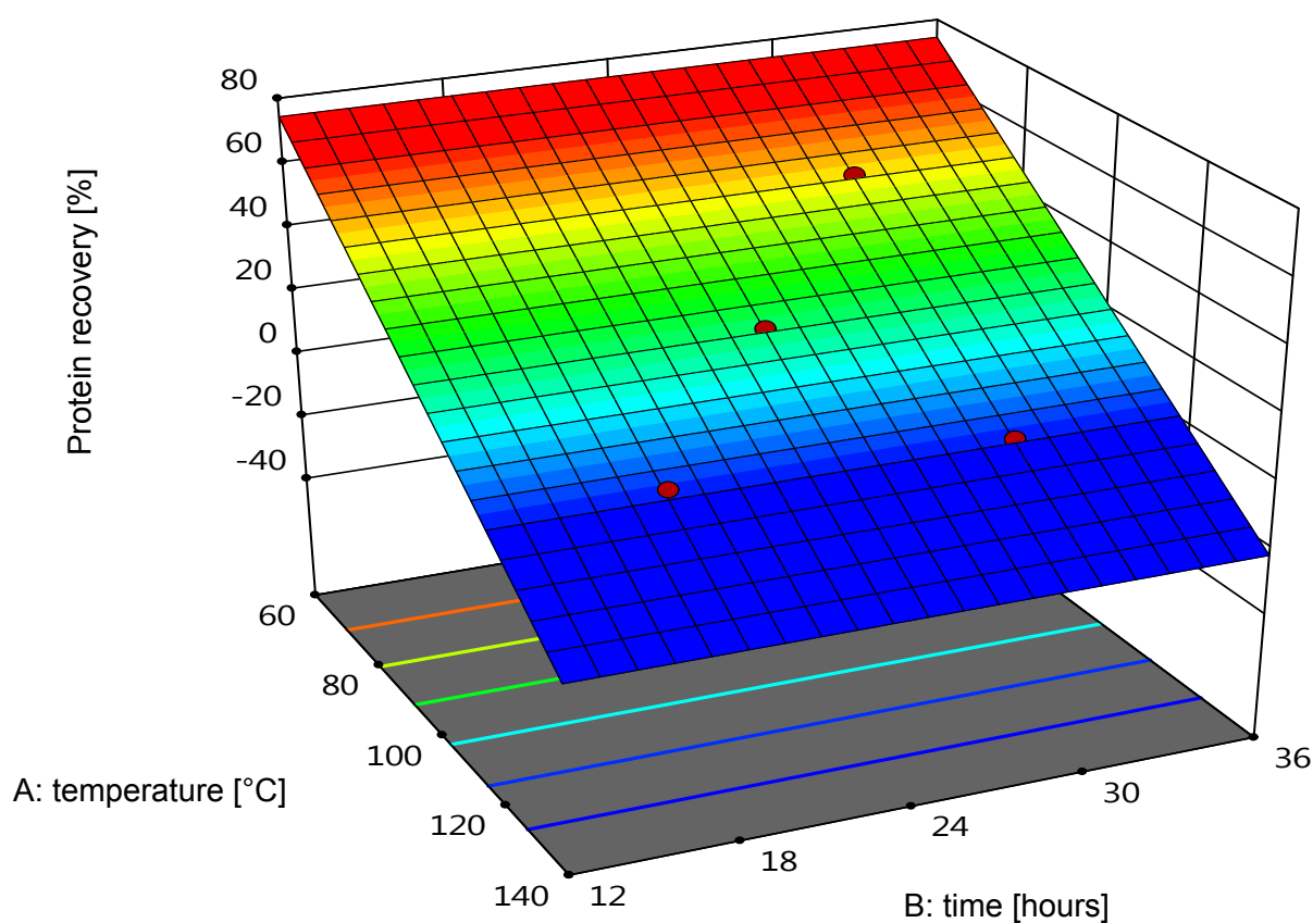
Figure 9: The 3D response surface for protein recovery as result of the Box-Behnken DoE. The red dots depict the run points above the surface.
