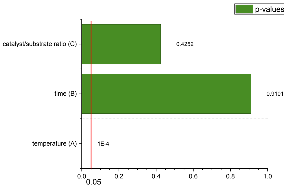
Figure 8: Pareto chart resulting of the Box-Behnken DoE for the linear model of the protein recovery. Red line indicates the significance limit of p = 0.05 which shows if the value is significant or not. A value below the significance level is significant.
