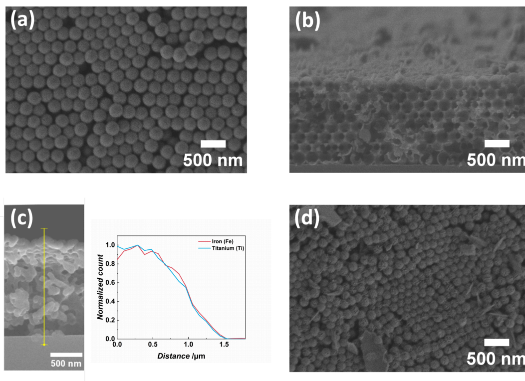
Figure 2. Characterization of the structural integrity and composition by SEM and EDX. (a) and (b) demonstrate the typical IO structure for (a) 16 nm \text{TiO}_2 IO and (b) 20 nm \text{TiO}_2 -2 nm \text{Fe}_2\text{O}_3 , both fabricated with 252 nm PS template size. (c) an EDX scan along a 20 nm \text{TiO}_2 -2 nm \text{Fe}_2\text{O}_3 cross-section reveals a homogeneous distribution of iron and titanium. (d) \text{Fe}_2\text{O}_3 -coated IOs present needle-like structures and larger particles at their top surface.
