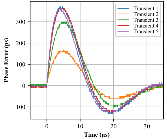
Fig. 5. Phase transients stimulated by broadbeam irradiation with ^{124}\text{Xe}^{35+} ions ( \text{LET}_{\text{Si}} = 62.5\ \text{MeV mg}^{-1}\text{cm}^2 ). Transients vary in peak amplitude but are very similar in temporal evolution. After the initial deviation from zero phase error up to about 5\ \mu\text{s} , the transient shape is determined by the active PLL control.
