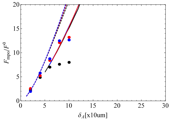
Fig. 9. Experimental results of the dynamic adhesion tests amplification of pull-off load F_{mpo}/F^0 , compared with the “exact” theory with solid lines (with a dynamic modulus estimated as K = 9.3 MPa, slightly higher than the relaxed one of 4 MPa): black, blue, red correspond to frequency \omega = 2\pi \times 200, 2\pi \times 300, 2\pi \times 400 rad/s for system parameters as all figures in this paper. (For interpretation of the references to color in this figure legend, the reader is referred to the web version of this article.)
