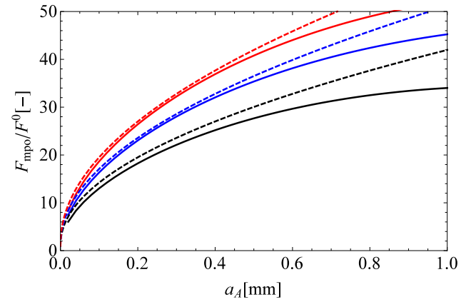
Fig. 7. The amplification of pull-off F_{mpo}/F^0 where F^0 = -3/2\pi R w_0 is pull-off in quasi-static conditions, as a function of the amplitude of oscillation of contact radius a_A . Solid black, blue, red correspond to frequency \omega = 2\pi \times 200, 2\pi \times 300, 2\pi \times 400 rad/s for system parameters as Fig. 2, and dashed line is our approximate solution (21) with corrected effective work of adhesion (24) with \beta = 2.5 . (For interpretation of the references to color in this figure legend, the reader is referred to the web version of this article.)
