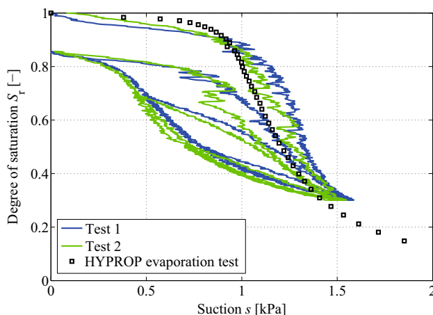
Fig. 7 Measured water retention curves from two hydraulic tests on Hamburg Sand with e_0 = 0.65 compared to water retention data from a HYPROP evaporation test
