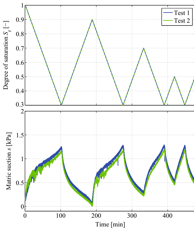
Fig. 8 Applied change of degree of saturation (top) and measured matric suction s [kPa] versus time from two hydraulic tests on glass beads with e_0 = 0.615 ( \frac{\partial V_w}{\partial t} = 0.0597 \frac{\text{mm}^3}{\text{s}} , \frac{\partial S_r}{\partial t} \approx 0.000116 \frac{1}{\text{s}} )
