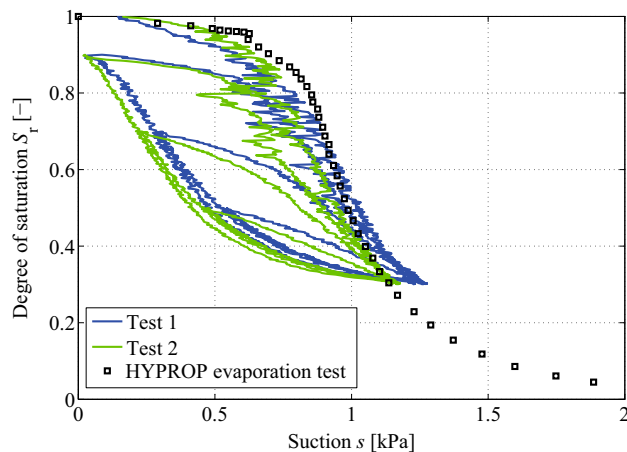
Fig. 9 Measured water retention curves from two hydraulic tests on glass beads with e_0 = 0.615 compared to water retention data from a HYPROP evaporation test
