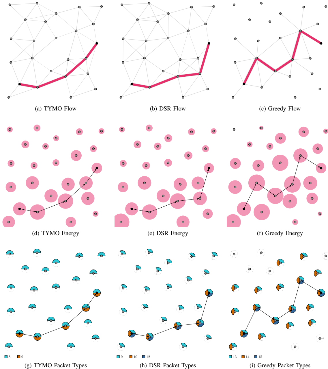
Fig. 11. Comparison between different routing protocols: packet flow, energy consumption and packet types
