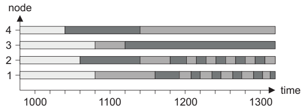
Fig. 7. A state tracing example.
