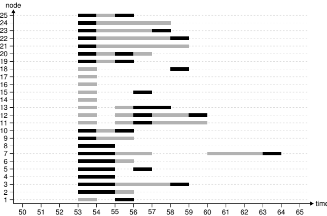
Fig. 10. State tracing of SelfWISE
