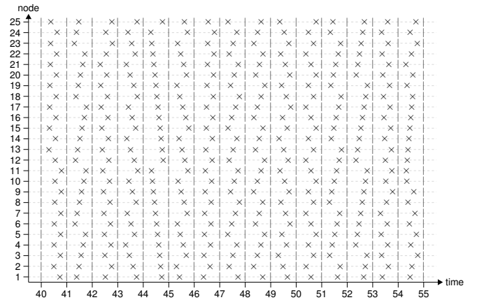
Fig. 9. Event tracing of SelfWISE
