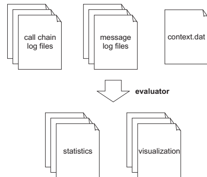
Fig. 5. Automated evaluation based on call chain and message log files.
