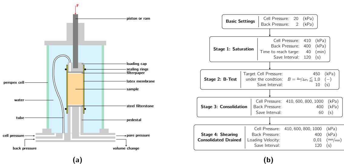
Figure 1: Triaxial testing device setup and test phases: (a) Device setup, (b) Test phases.
