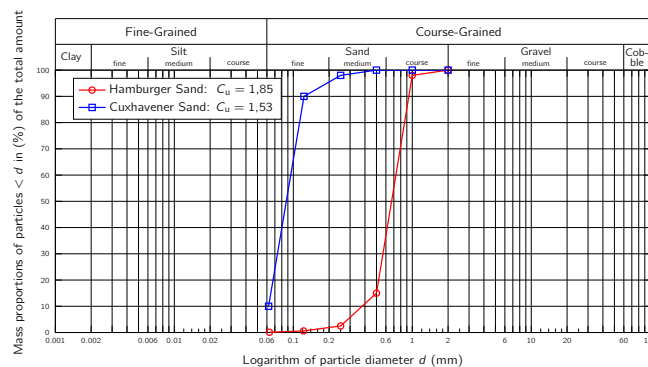
Figure 2: Grain Size Distributions of the Hamburg and Cuxhaven Sand
