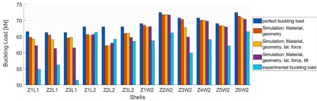
Fig. 12. Numerical buckling loads for different model setups.
