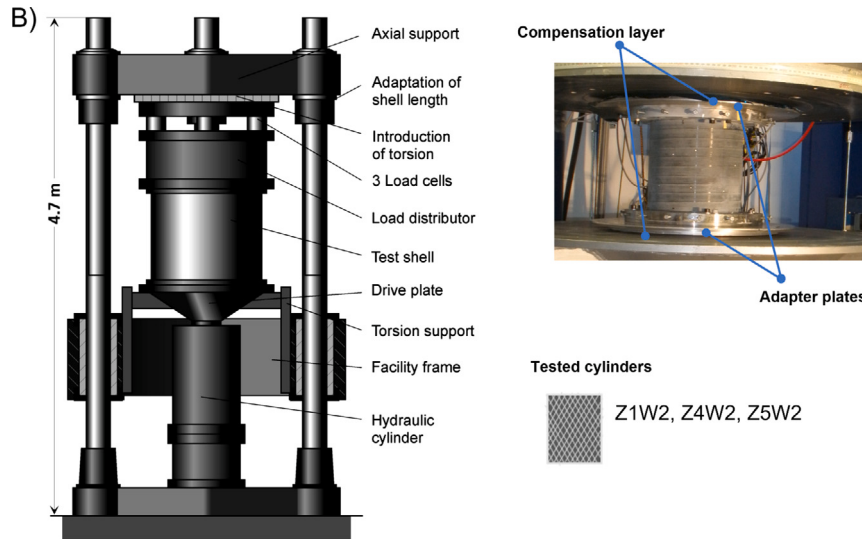
Fig. 2. Test setup of the DLR buckling facility.
