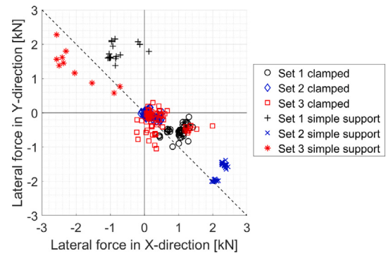
Fig. 6. Measured lateral forces before buckling in the Hexapod coordinate system.
