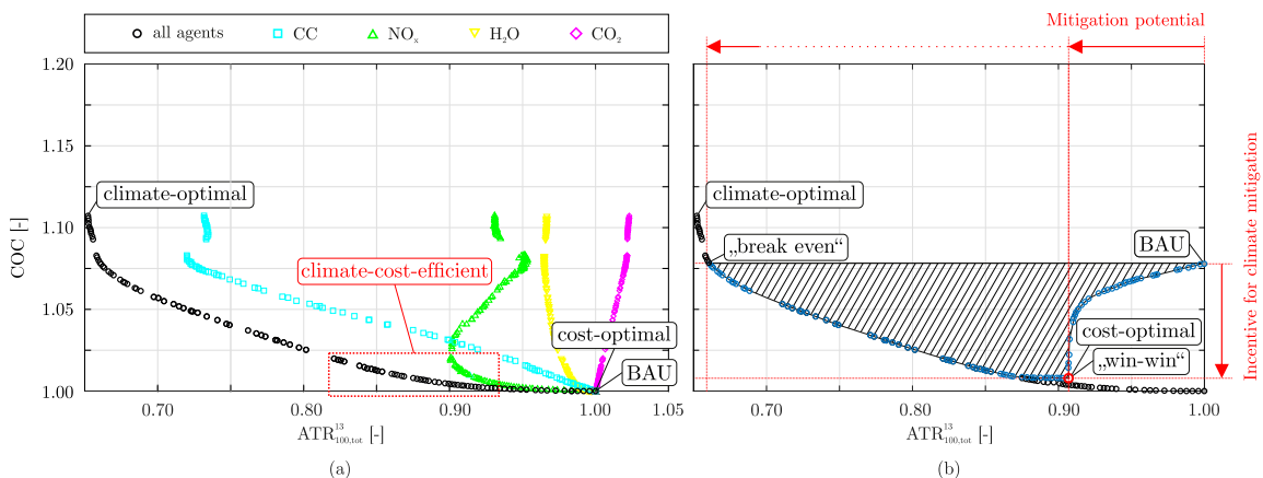
Figure 8. Climate mitigation potential (in ATR) and cash operating costs (COC) of (a) COTs and (b) the CCA concept (blue circles) on the transatlantic route LIS-MIA, assuming a climate unit charge of 1 $/km, a threshold of 0.664, and no wind effects.
