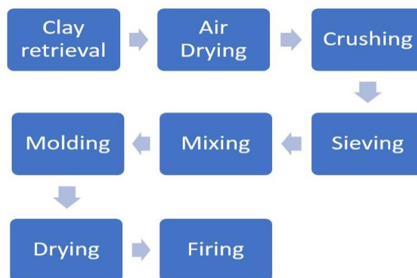
Fig. 2 Manufacturing process for clay cups
