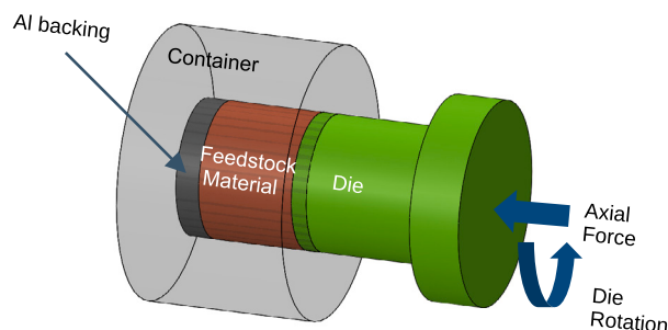
Fig. 1. Schematic illustration of the FC process.
