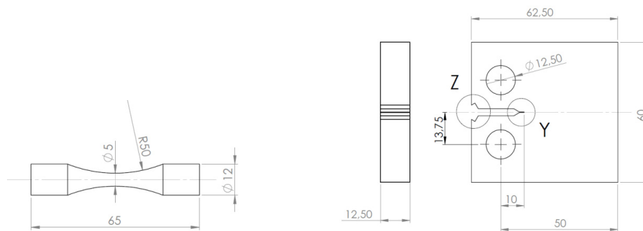
Fig. 1. Hour-glass shaped specimen for HCF tests (left) and CT-specimen for crack propagation tests (right).
