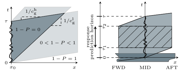
(a) Construction of the prediction zone (b) Definition of the response prediction horizon
