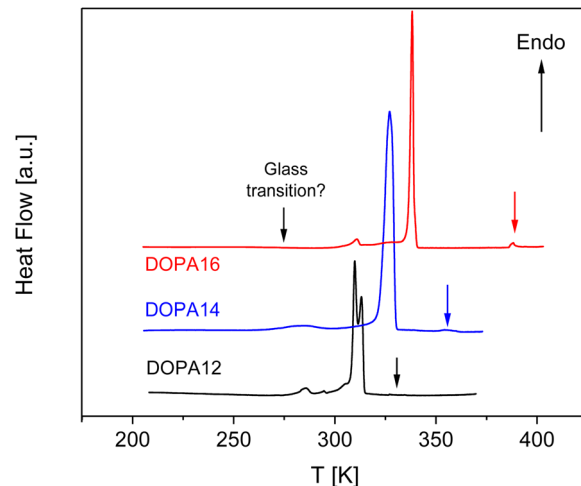
Fig. 3 Heat flow versus temperature for the considered ionic liquid crystals (second heating run, heating rate 5 \text{ K min}^{-1} ): black – DOPA12, blue – DOPA14, red – DOPA16. The curves are shifted along the y-scale for sake of clarity. The phase transition from the \text{Col}_h to the isotropic state is marked by down sited arrows.
