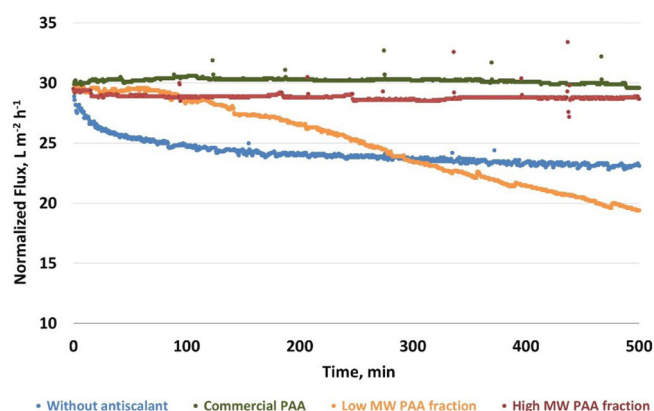
Fig. 3 | Flux behavior in the lab-scale RO experiments during calcite scaling. Flat sheet RO membrane operated with 22 mM \text{NaHCO}_3 and \text{CaCl}_2 feed and commercial PAA and its low and high MW fractions (Antiscalant dosing as 0.5 \text{ mg TOC L}^{-1} in each experiment); TMP = 25 bar, complete recirculation mode, T = 11^\circ\text{C} , \text{SI}_{\text{calcite}} \approx 1.09 .
