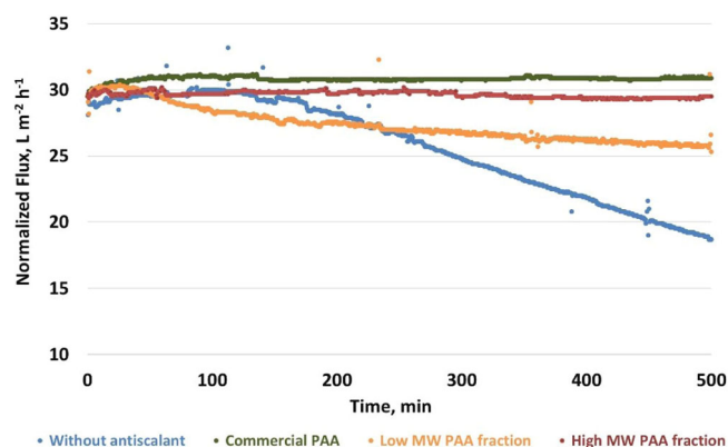
Fig. 2 | Flux behavior in the lab-scale RO experiments during gypsum scaling. Flat sheet RO membrane operated with 25 mM \text{Na}_2\text{SO}_4 and \text{CaCl}_2 feed and commercial PAA and its low and high MW fractions (Antiscalant dosing as 0.5 \text{ mg TOC L}^{-1} in each experiment); TMP = 25 bar, complete recirculation mode, T = 11^\circ\text{C} , \text{SI}_{\text{gypsum}} \approx 0.2 .
