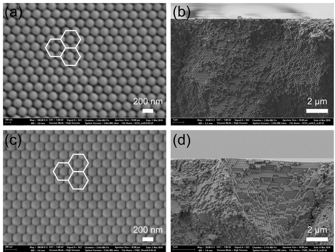
Figure 4. The structures of the prepared opal without (a,b) and with (c,d) conformal coating of TiO 2 . Top view (a) and cross-sectional (b) SEM images of the opal without conformal coating. Top view (c) and cross-sectional (d) SEM images of the opal with 19.1 nm (full infiltration) TiO 2 conformal coating. The white hexagons in image (a,c) illustrate the close-packing and the {111} planes.
