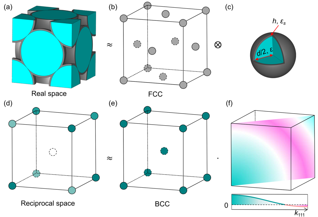
Figure 1. A conformally coated opal is schematically illustrated in real and reciprocal space. In real space the structure (a) can be seen as the convolution of the FCC lattice (b) with the motif (c). The motif can be simplified to a core-shell sphere by neglecting the contact points between spheres. Accordingly, the total FT of the structure (d) can be written as multiplication of the lattice FT (e) and the motif FT (f) where the amplitude distribution on the {110} plane is further shown.
