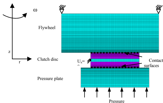
Fig. 6. FE models with the boundary conditions.
