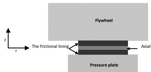
Fig. 3. The Contact model for clutch system.
