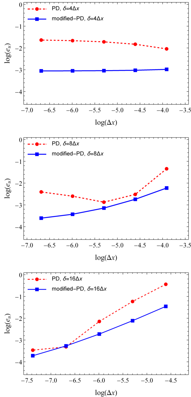
FIGURE 6 | \delta -convergence study for Example 1: \log(e_u) versus \log(\Delta x) for PD (red, dashed) and modified-PD (blue, solid) with m_{\text{ratio}} \in \{4, 8, 16\} .
