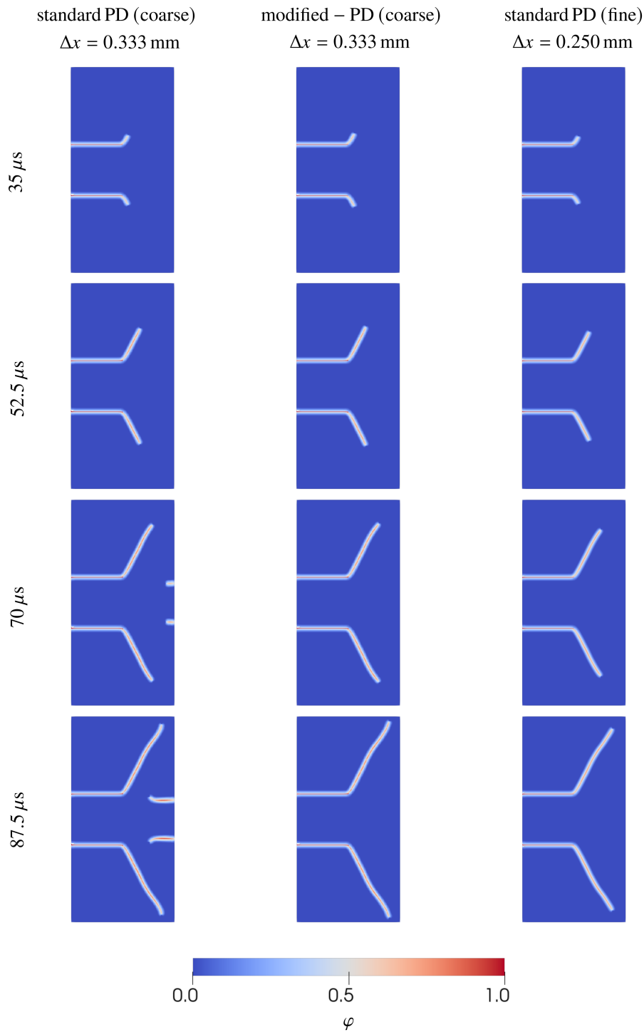
FIGURE 17 | Damage evolution at t \in \{35, 52.5, 70, 87.5\} \mu s. Columns: standard PD (coarse) ( \Delta x = 0.333 mm), modified-PD (coarse) ( \Delta x = 0.333 mm), and standard PD (fine) ( \Delta x = 0.250 mm), all with \delta = 4 mm.
